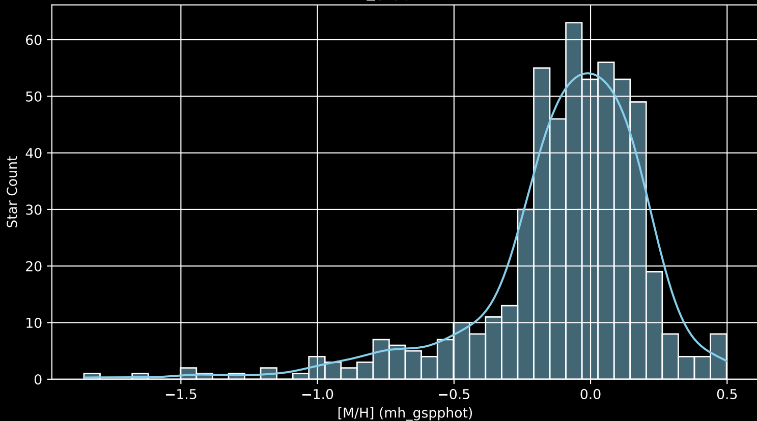
APOGEE DR17 Field: [100+12 [M/H] (mh_gspphot) (n= 540)
