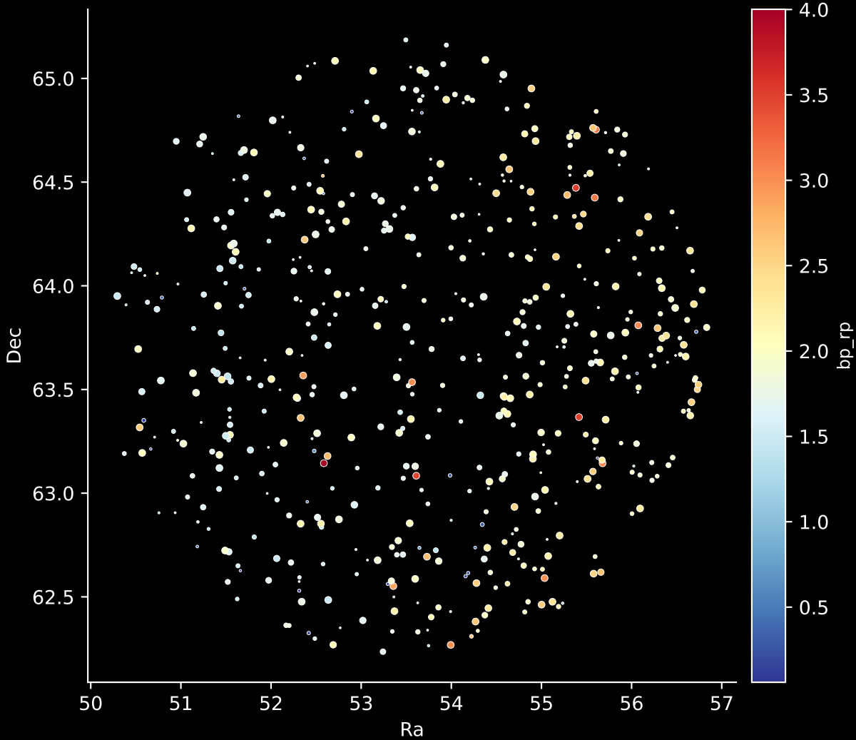
APOGEE DR17 Field: [100+12] Stars: 547
