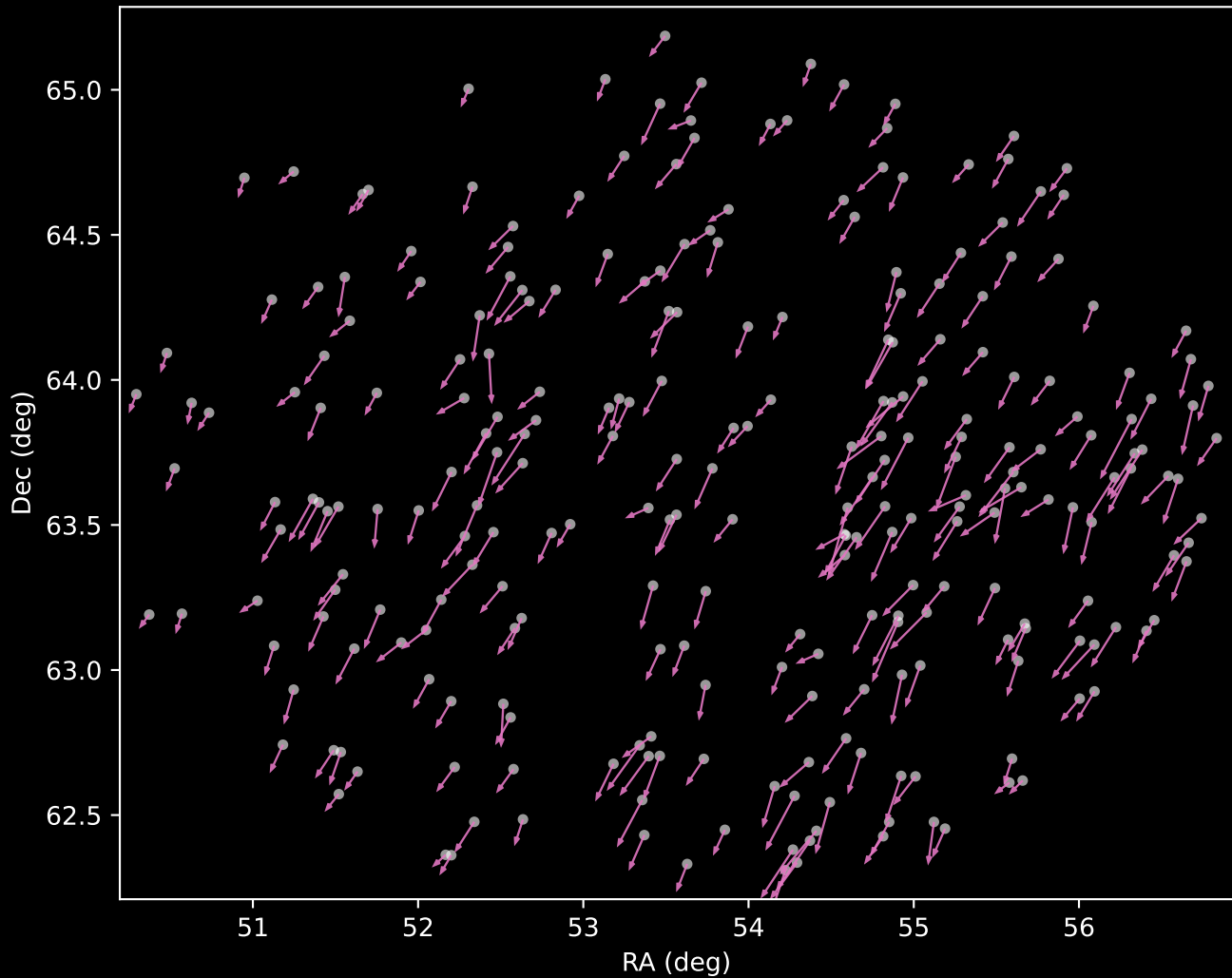
APOGEE DR17 Cluster 12 Proper Motion Vectors (n=262)
