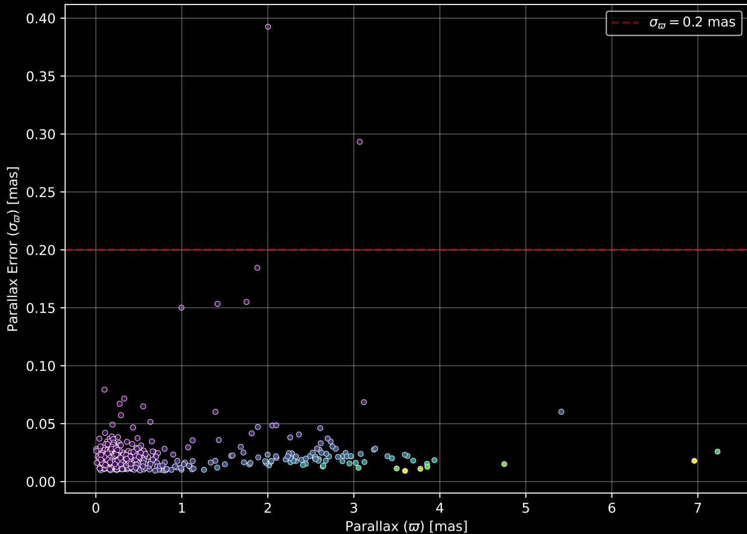
APOGEE DR17 Field: [100+12] Parallax Quality (n= 547)
