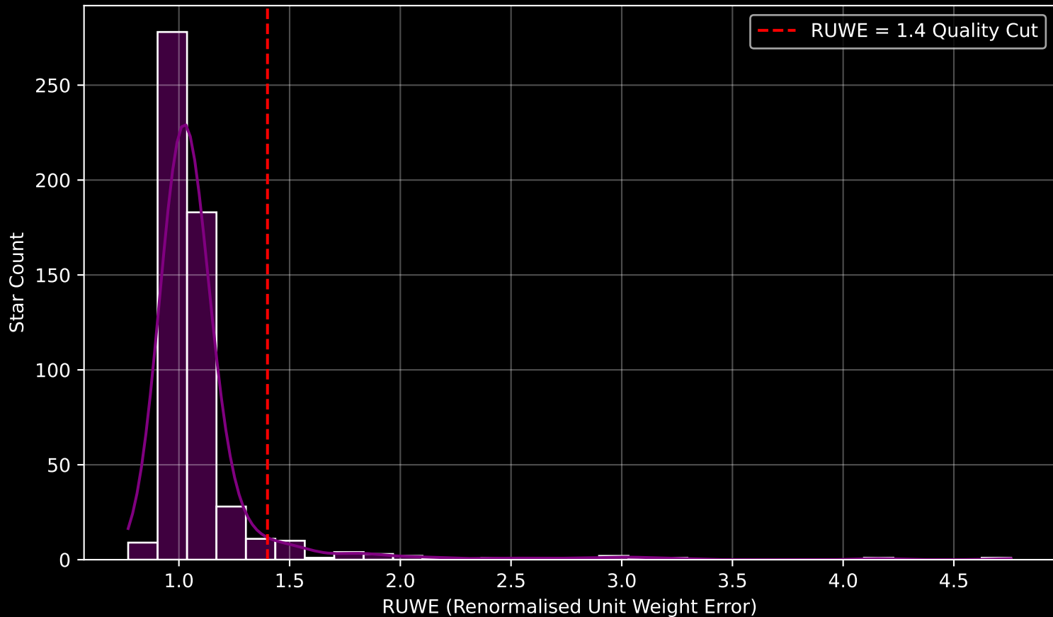
GAPOGEE DR17 Field [100+12] RUWE Distribution (n= 539)
