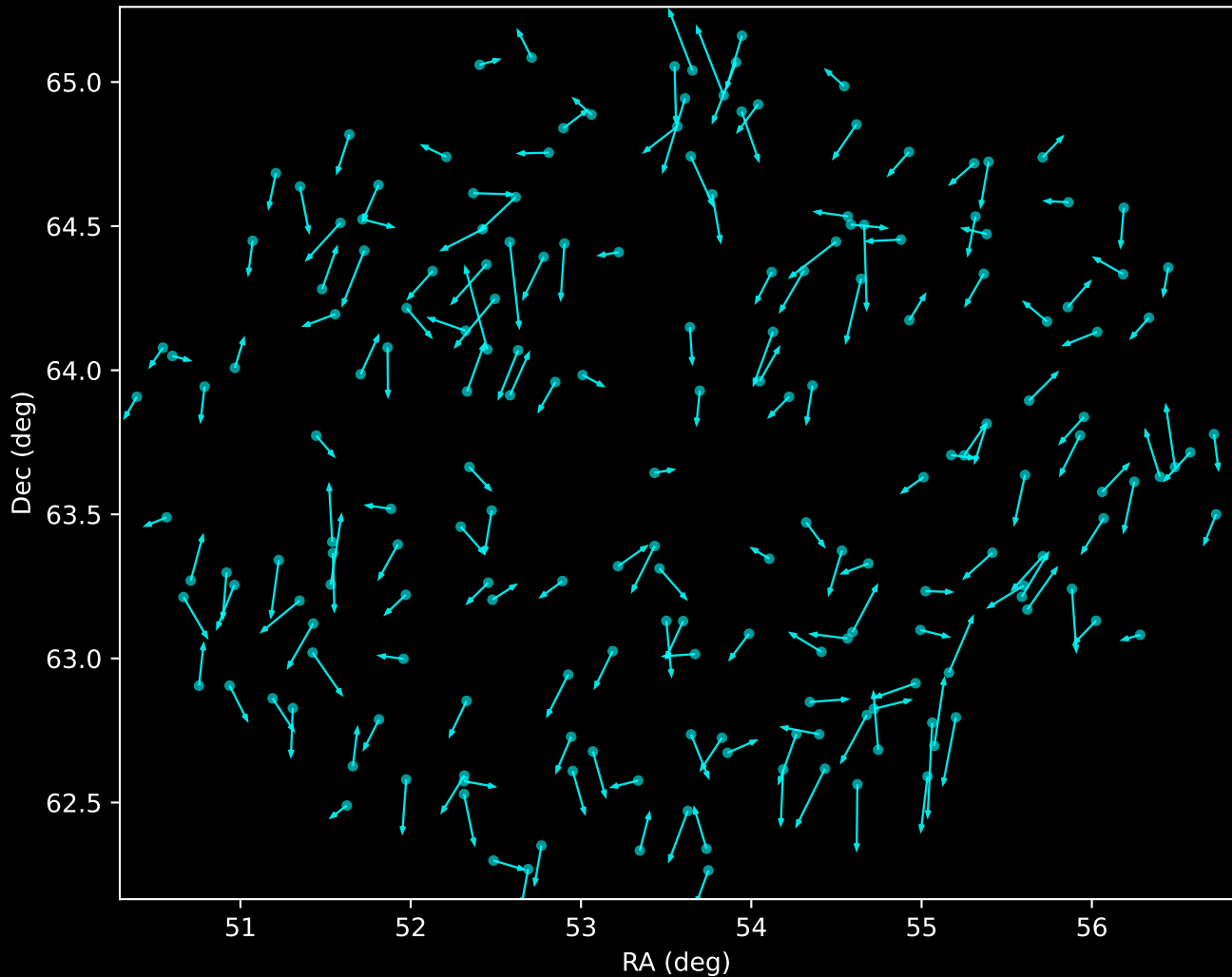
APOGEE DR17 Noise Stream Proper Motion Vectors (n=191)
