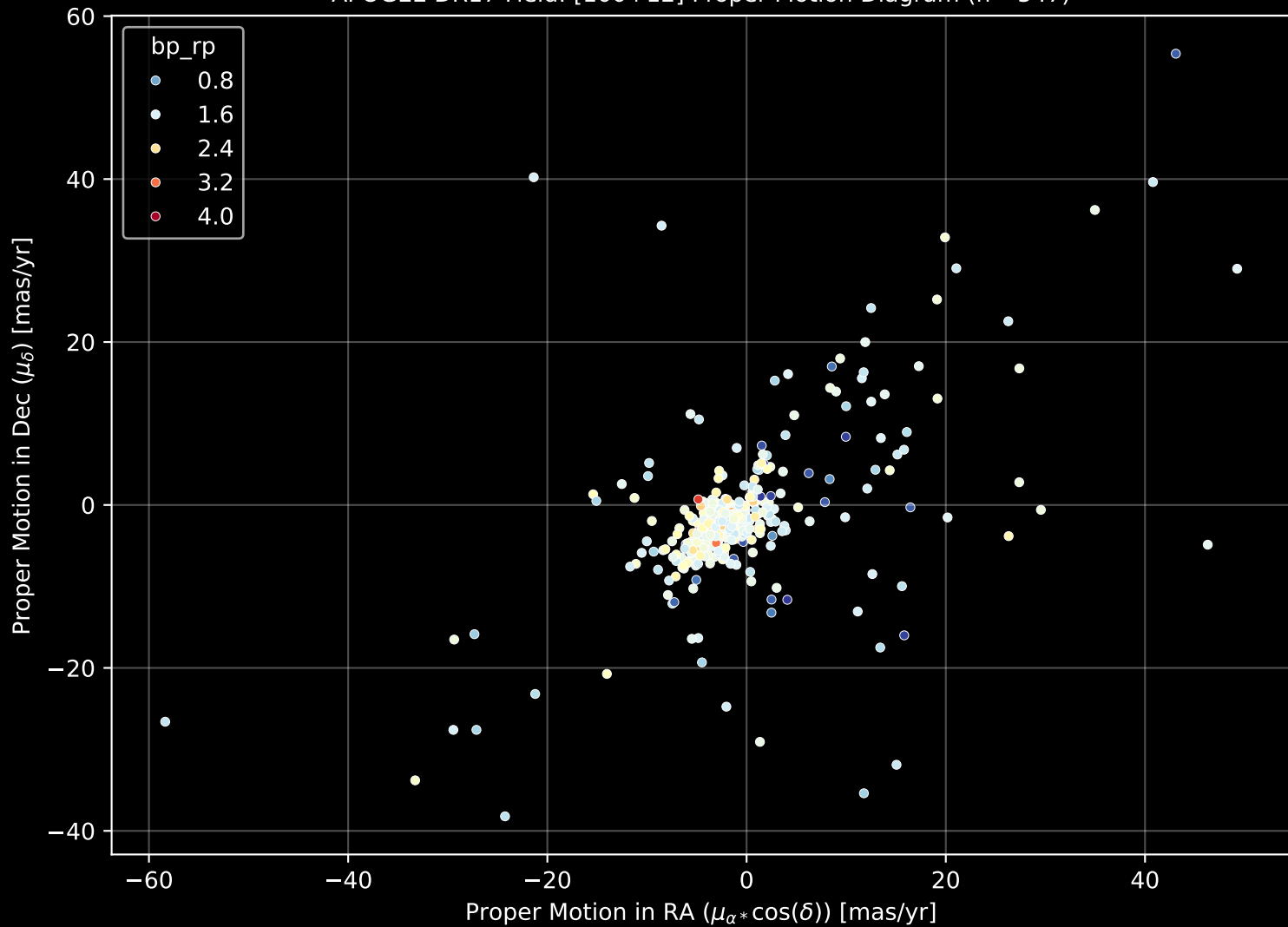
APOGEE DR17 Field: [100+12] Proper Motion Diagram (n= 547)
